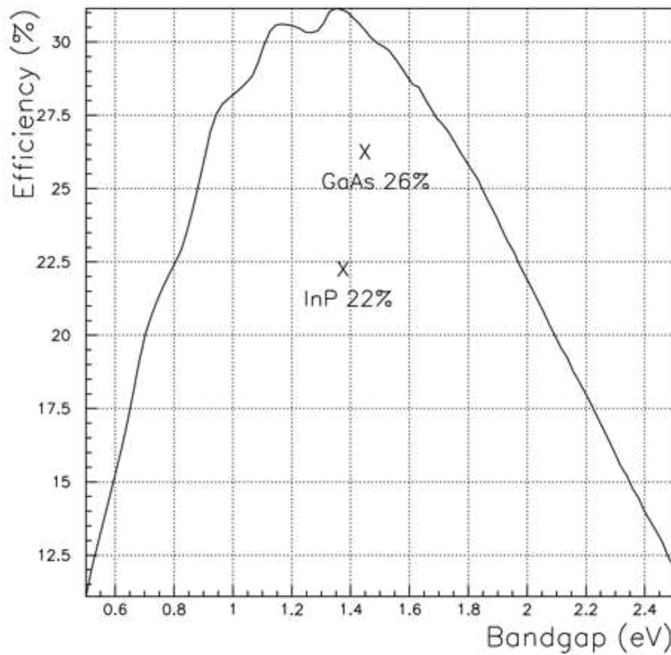
Figure 4 Single junction solar cell ideal conversion efficiency in the radiative limit as a function of bandgap showing best single junction results to date for two key III-V semiconductors. Both have bandgaps close to the optimum of 1.35eV with a potential conversion efficiency of 31.1% for an ideal cell with only radiative recombination losses.
