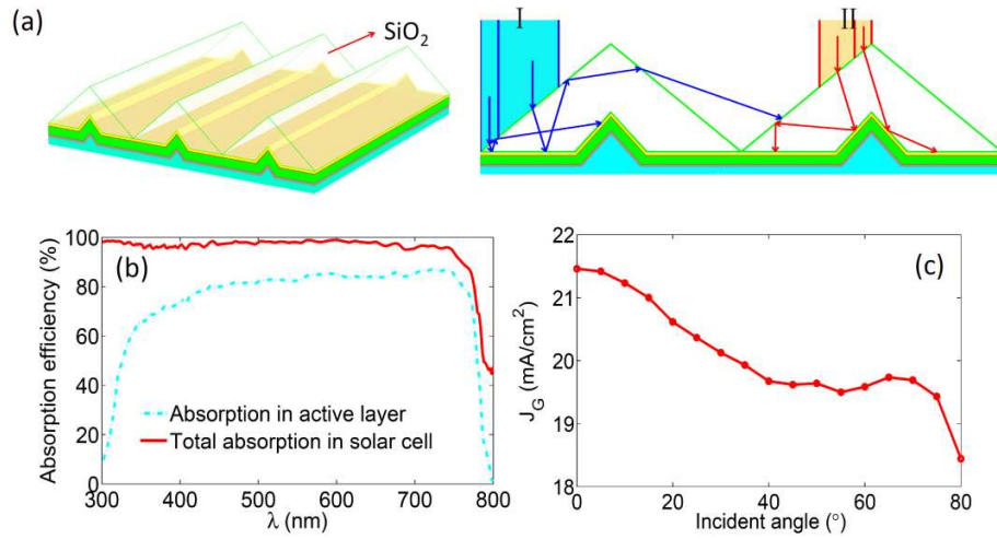
Figure 3 | Schematic of light trapping induced by slotted SiO 2 prism structures and corresponding optical property of the solar cell. (a) The schematic of the perovskite solar cell with slotted SiO 2 prism structures and traveling path of the incident light from different regions. (b) The absorption efficiency for total and the active layer. (c) The photo-generated current ( J_G ) as function of the incident angle.
